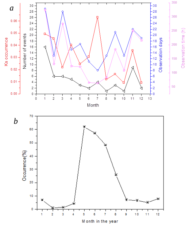
Figure 3. Seasonal distributions of K_s occurrence (frequency and numbers) at our location and the observation time (days and hours) in each month ( a ); seasonal distribution of E_s occurrence ( b )
