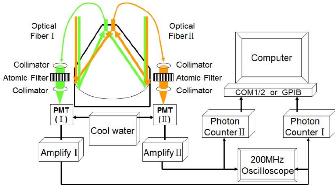
Figure 1. Lidar system
