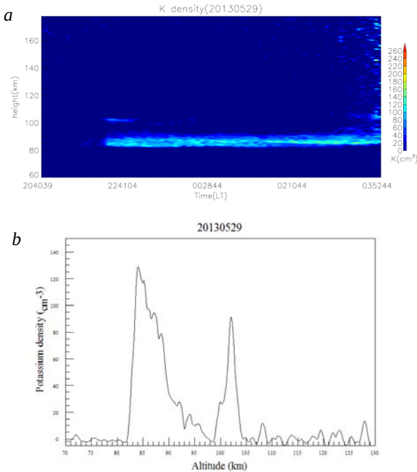
Figure 2. Contour of the K layer observed at the Beijing site from 20:40:39 LT on May 29, 2013 to 03:52:44 LT on May 30, 2013 ( a ); the K density profile observed at 23:16 LT ( b )
