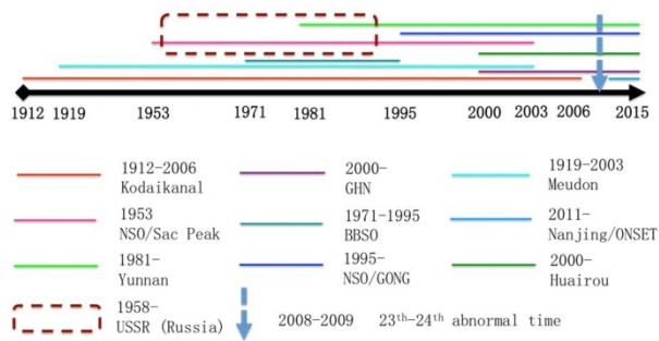
Figure. Ha observing time coverage
