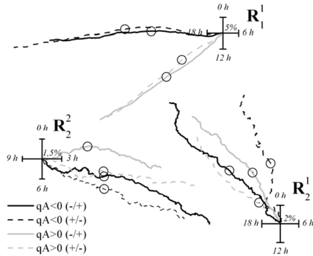
Figure 3. Behavior of R_1^1 , R_2^1 , and R_2^2 4 days before and 5 days after the NCS crossings. Crossings of different types are marked with different colors and lines. Circles are moments of the crossings
