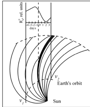
Figure 2. Scheme of interaction between slow and fast SW streams, where v_1 and v_2 are the speeds of catching-up and fall-ing-down sectors such that v_1 > v_2 . In addition, the expected isotropic intensity R_0^0 is shown
