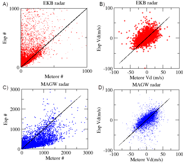
Figure 7. Relationship between the number of scattered signals (a, c) and hourly average velocities (b, d) in classes 13 (meteor echo) and 2 (sporadic scattering) as recorded by the EKB (a, b) and MAGW (c, d) radars
