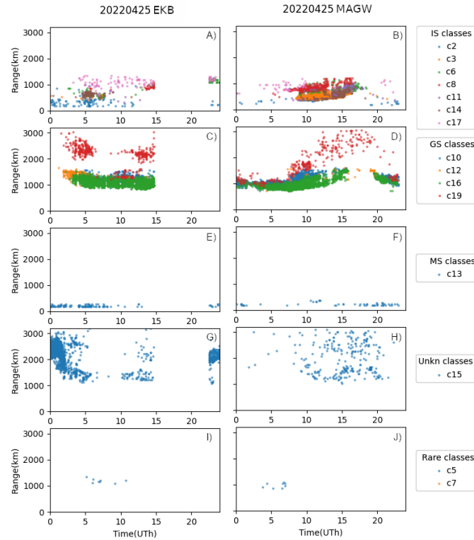
Figure 3. Example of operation of the algorithm using ISTP SB RAS data from EKB (left) and MAGW (right) radars on April 25, 2022. From top to bottom: ionospheric scattering classes (a, b); groundscattering classes (c, d); meteor scattering classes (e, f); unidentified classes (g, h); rarely observed classes (i, j)
