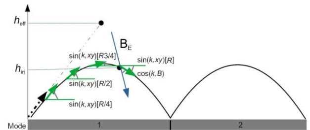
Figure 1. Scheme of calculation of physical parameters determined by numerical simulation. The solid black line is the radio signal propagation path calculated using ray tracing. The blue arrow is the geomagnetic field direction; horizontal green lines mark the horizon direction; green solid arrows, the radio signal propagation direction
