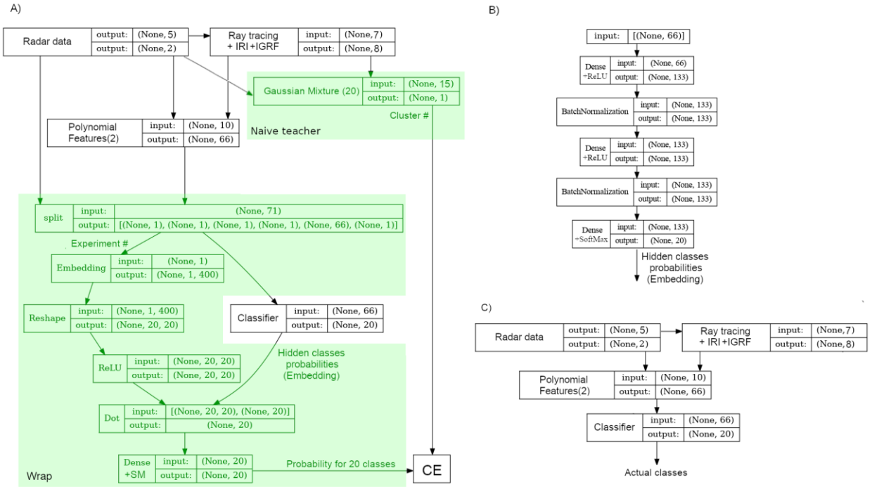
Figure 2. Architecture of the Wrapped Classifier with Naive Teacher and vector dimensions: network architecture in learn mode (a); classifier architecture (b); network architecture in processing mode (c). "None" stands for the number of records in the dataset
