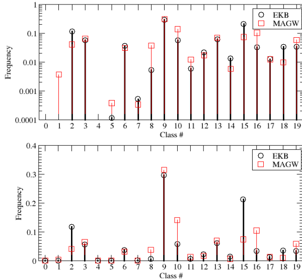
Figure 4. Frequency distribution of observed signal classes in the EKB and MAGW ISTP SB RAS data during training on logarithmic (top) and linear (bottom) scales
