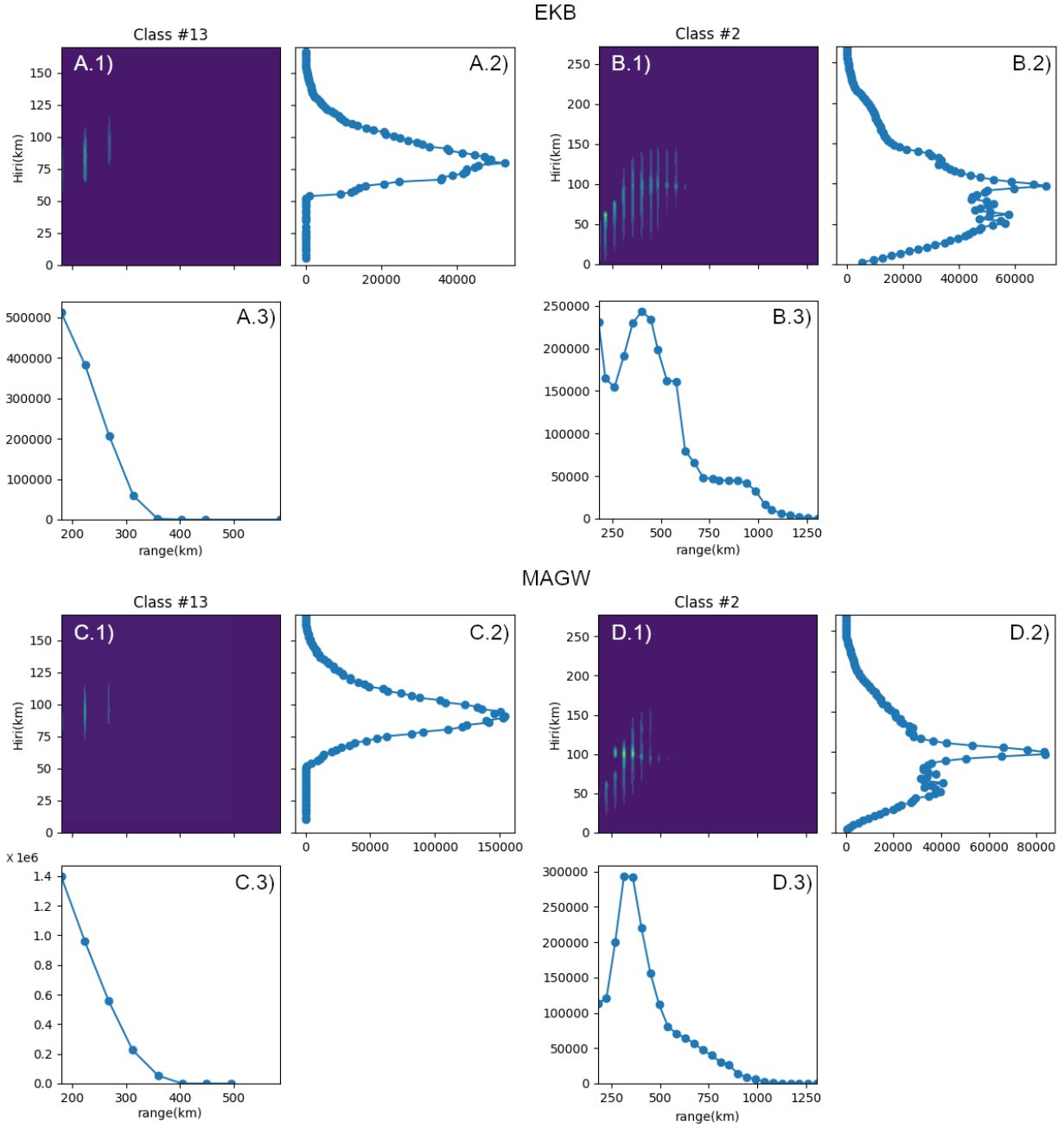
Figure 5. Comparison of altitude-range distributions of classes 13 and 2 for January 2021 – March 2022. Altitude-range distribution of the rate of observation of traces ( a1–d1 ); rate of occurrence of scatterers depending on the height calculated from signal propagation path ( a2–d2 ); signal distribution as a function of radar range ( a3–d3 )
