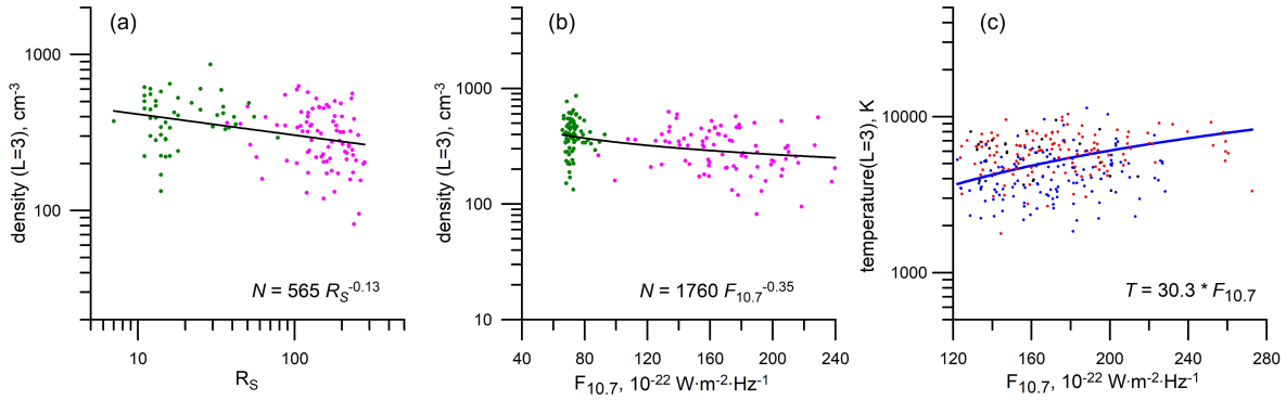
Figure 4. Proton density (a, b) and temperature (c), measured by Interball-1 (a, b) and Magion-5 (c) in the plane of the magnetic equator of the plasmasphere, as function of the solar activity indices R_s (a) and F_{10.7} (b, c). Measurements at solar minimum (1995–1997) are highlighted in green in the left panels (a, b); measurements at solar maximum (1999–2000), in purple. In the right panel (c), daytime measurements (06–18 MLT) are shown in red; and nighttime measurements (18–06 MLT), in blue
