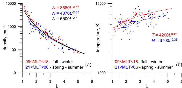
Figure 1. Proton density (a) and temperature (b) measured by Interball-1 in the plane of the magnetic equator of the plasmasphere for two MLT intervals (daytime hours 09:00–18:00 (red dots) and night hours 21:00–06:00 (blue dots)), as function of the distance to the center of Earth. The corresponding power-law approximations are highlighted in the same colors. The black curve in panel a indicates general approximation (2)
