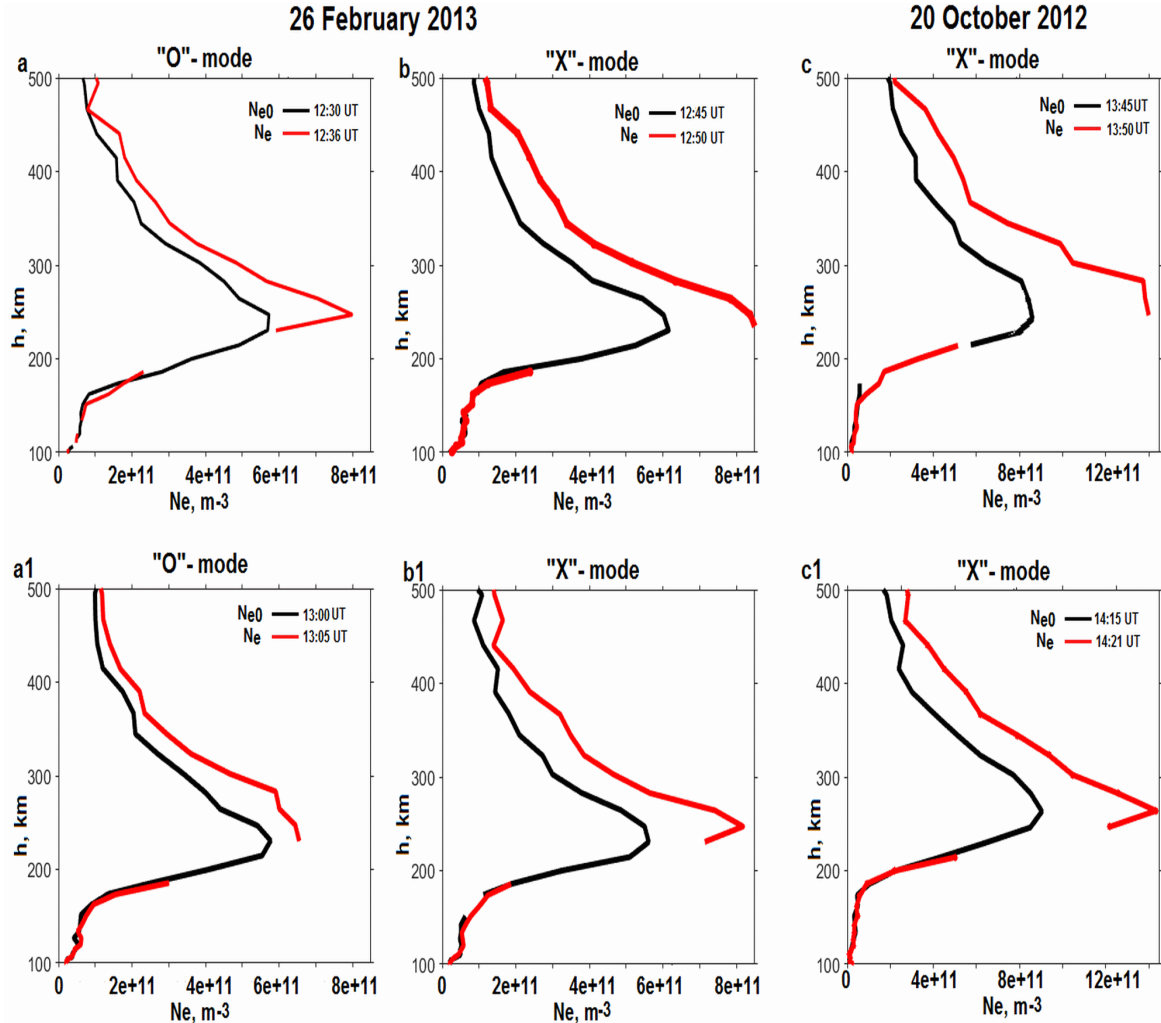
Figure 3. Electron density profiles as a function of height of the high-latitude ionosphere as derived from EISCAT radar data before the heating cycles ( N_{e0} , black) and during the heating periods with 100 % ERP ( N_e , red): February 26, 2013, f_H/f_oF2 \sim 1 for O-mode HF heating cycles 12:31–12:41 UT (a) and 13:01–13:11 UT (a1) and X-mode HF heating cycles 12:46–12:56 UT (b) and 13:16–13:26 UT (b1); October 20, 2012, f_H/f_oF2 < 1 for X-mode HF heating cycles 13:46–13:56 UT (c) and 14:16–14:26 UT (c1) (no N_e increase was recorded at O-mode HF heating)
