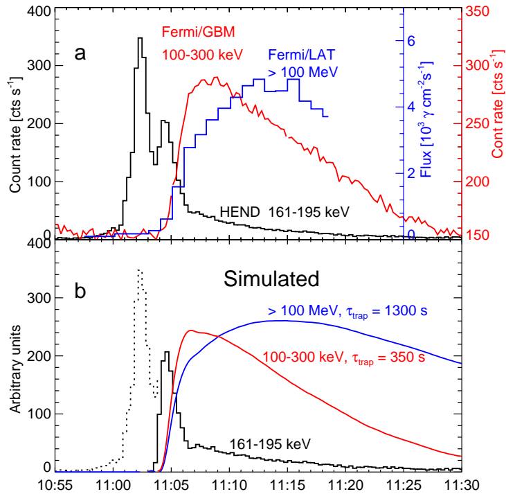
Figure 11. The trapping effect issue. a) Hard emissions actually observed (corresponding to Figure 3): 161–195 keV flare hard X-rays ( Mars Odyssey /HEND, black), 100–300 keV viewed from the Earth’s direction ( Fermi /GBM, red), and > 100 MeV \gamma -ray burst ( Fermi /LAT, thick-blue). The one-second and four-second time-resolution Fermi /GBM data are both summed over 16 seconds for convenience. b) Simulated temporal profiles expected as a result of trapping: the injection function for the second HXR peak [ f_{inj} ] (black-solid), actual HXR temporal profile (black-dotted), and simulated emissions from trapped electrons (red) and protons (thick-blue).
