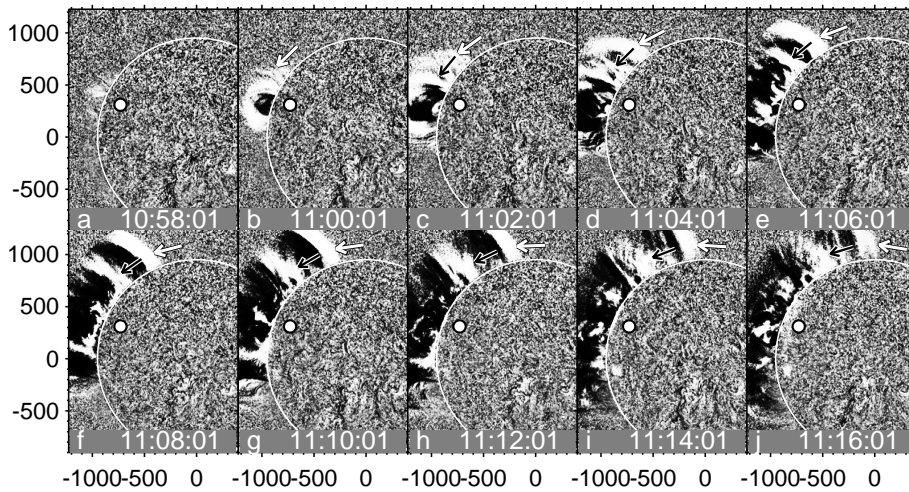
Figure 7. EUV wave propagation along the limb observed in running-difference AIA 211 Å images. The arrows point at the first (white arrow) and second (black arrow) EUV wave fronts. The white dot denotes the projected position of the flare site. The axes show the distances from solar disk center in arcseconds. The temporal interval between all consecutive images is two minutes.
