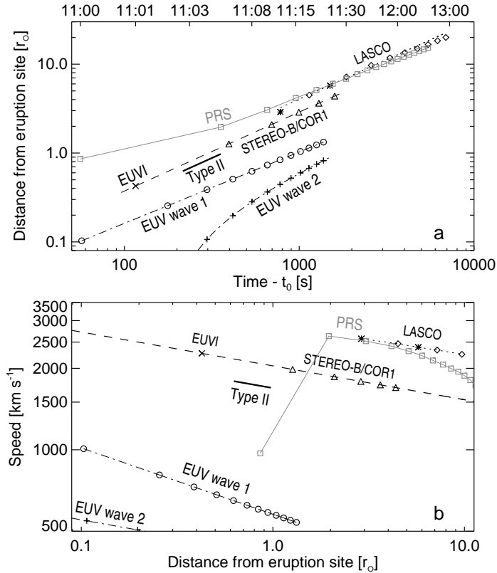
Figure 10. Decelerating power-law kinematics of the shock waves measured from different vantage points using different methods. All distances are measured from the eruption center located at 0.84 R_{\odot} . a) Distance–time plots. The horizontal axis represents time after the wave onset t_{01} = 10:59:04 in the logarithmic scale. The upper X -axis shows actual times. b) Speed–distance plots. The symbols represent our measurements from the images produced by different telescopes. The measurements from the CME catalog are shown by asterisks (C2) and diamonds (C3). The thick bar represents the shock kinematics corresponding to possible Type II bands outlined in the dynamic spectrum. The gray squares denoted “PRS” represent the measurements from Plotnikov, Rouillard, and Share (2017). The black lines of different styles show the analytic fit.
